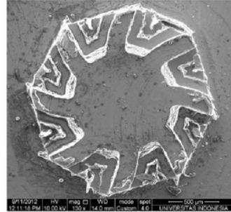
Fig.5. Micro-impeller with diameter of 2 mm developed with depth per-cut, spindle speed and feed-rate of 10 μm, 80,000 RPM, and 60 mm/min, respectively.
