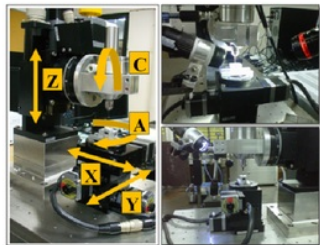
Fig.1. Micro-milling machine, Hadaia micromill-5X
