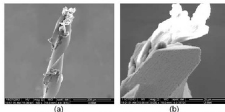
Fig. 2 Unacceptable micro-tool conditions (a) 500X (b) 5,000X
