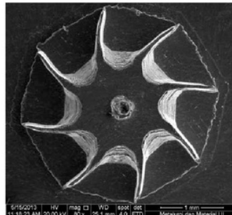
Fig.6. Micro-impeller with diameter of 3 mm developed with depth per-cut, spindle speed and feed-rate of 10 mm, 70,000 RPM and 30 mm/min, respectively.
